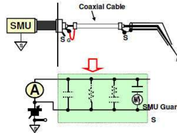
Coaxial cable
