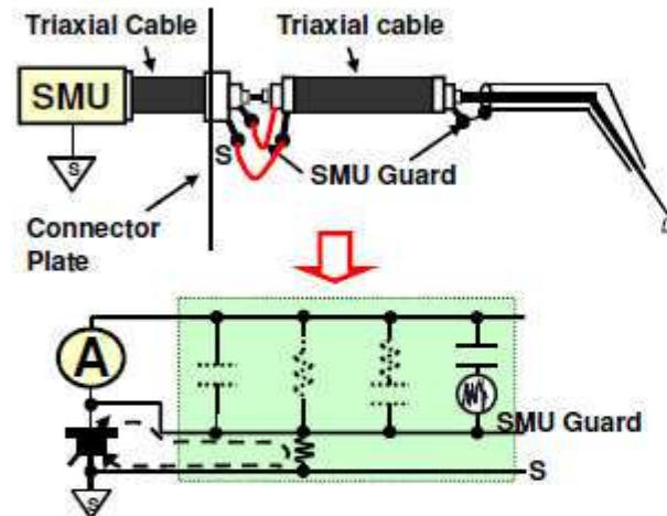
Triaxial Cable
