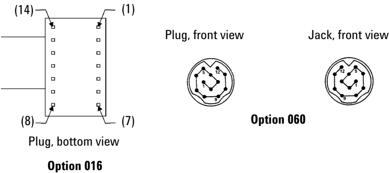
Figure 3 Solenoid Cable Pin Configuration
